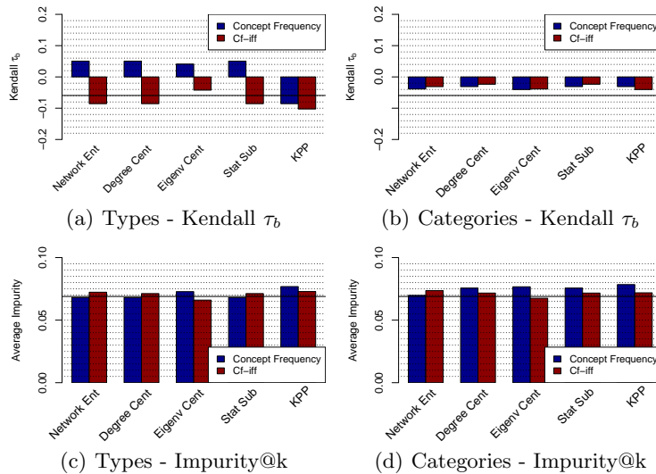
Fig. 2. Plots of the results obtained when measuring forum specificity using: a) the DBPedia type graph, and b) the DBPedia SKOS Category graph. The black horizontal line indicates the performance of the Knuth Shuffle random baseline.
